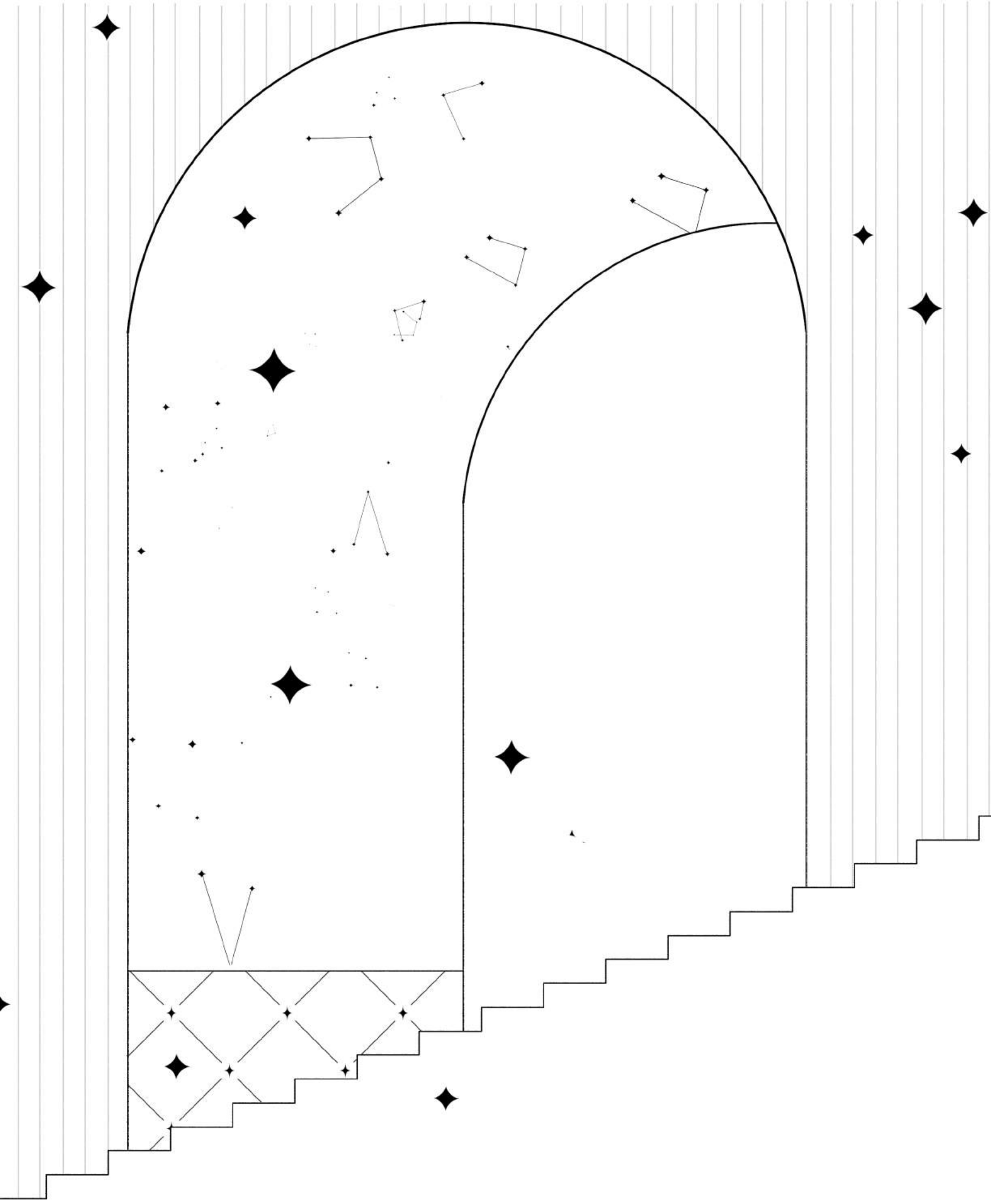
ORION'S BELT
